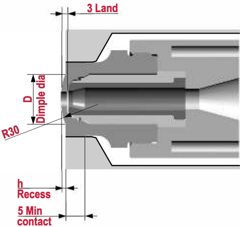
Spherical Recess
