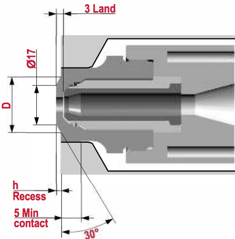
Conical Recess
