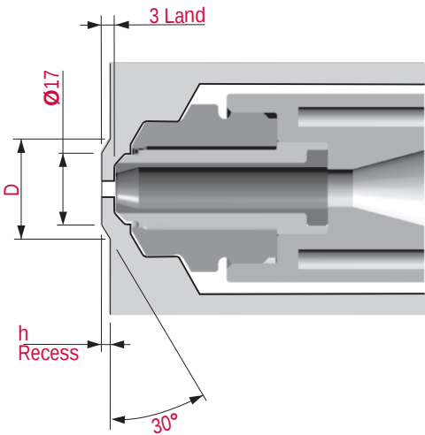
Conical Recess
