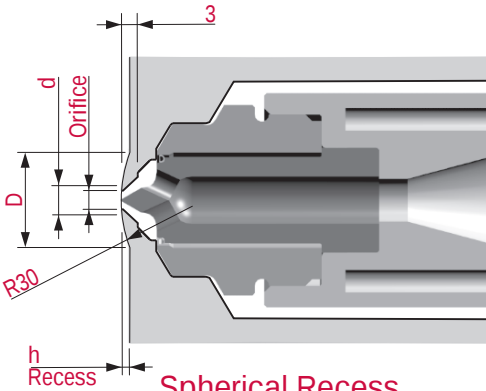
Spherical Recess
