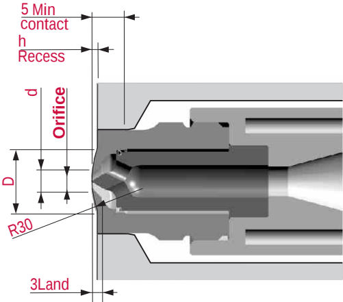
Spherical Recess
