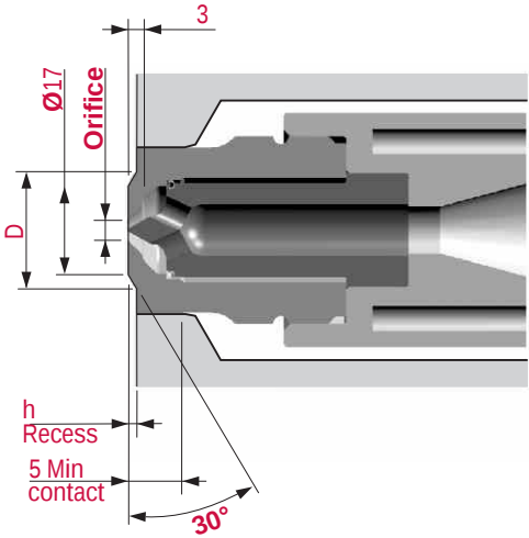
Conical Recess
