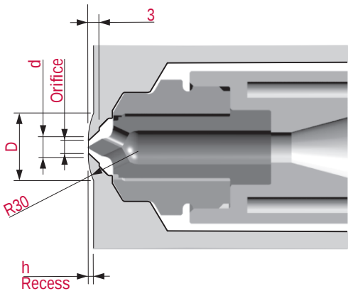
Spherical Recess
