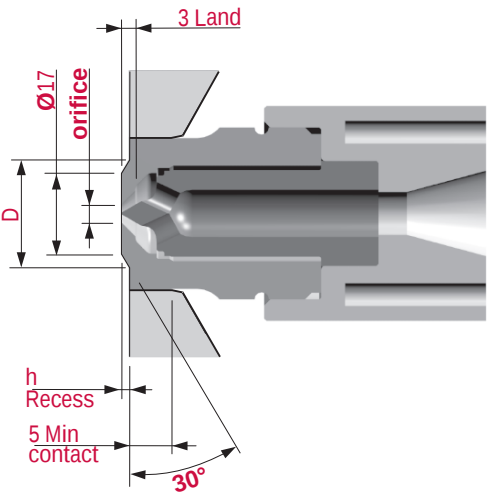
Conical Recess
