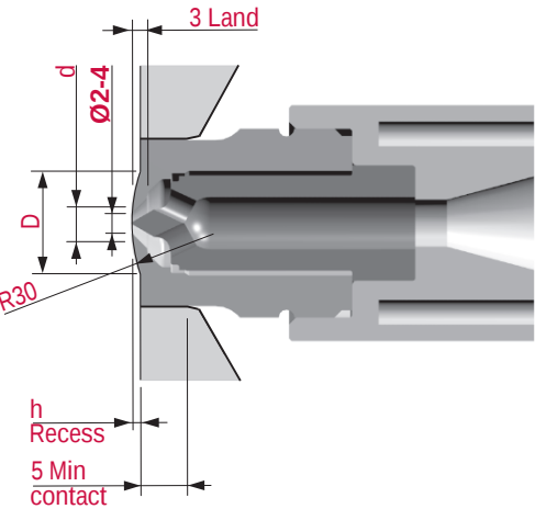
Spherical Recess
