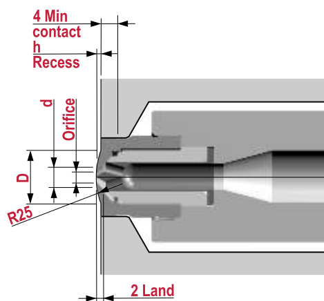
Spherical Recess
