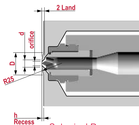
Spherical Recess
