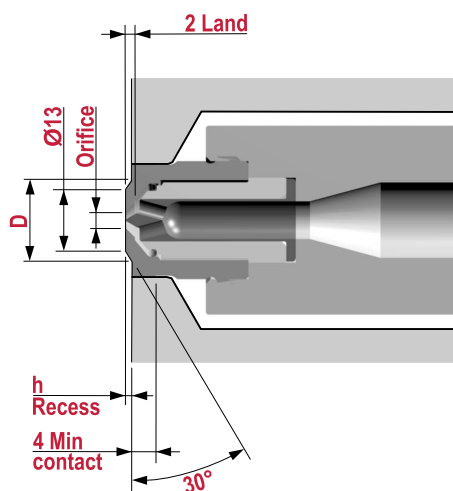
Conical Recess
