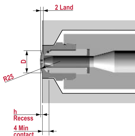
Spherical Recess
