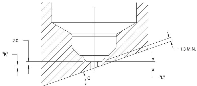
ANGLED MOLD CONTOUR
