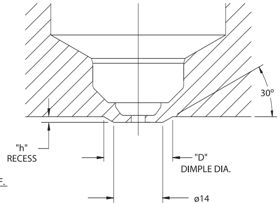
CONICAL GATE RECESS
