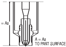
GATING ONTO A FLAT SURFACE
