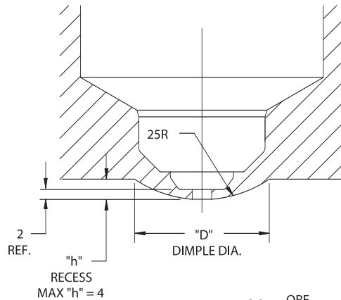
SPHERICAL GATE RECESS
